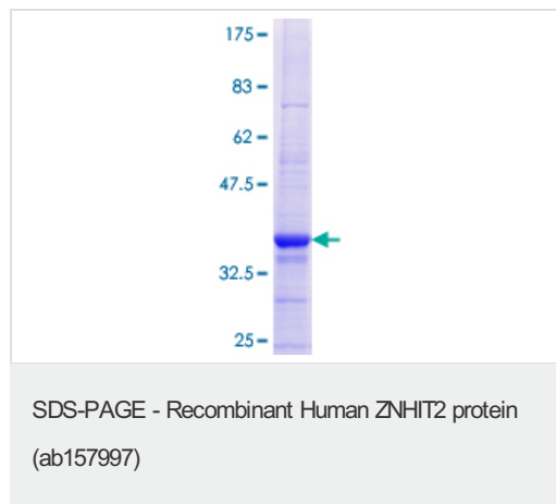
ab157997 on a 12.5% SDS-PAGE stained with Coomassie Blue.
