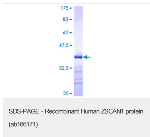
ab166171 on a 12.5% SDS-PAGE stained with Coomassie Blue.
