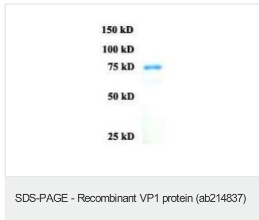
SDS-PAGE analysis of ab214837.
