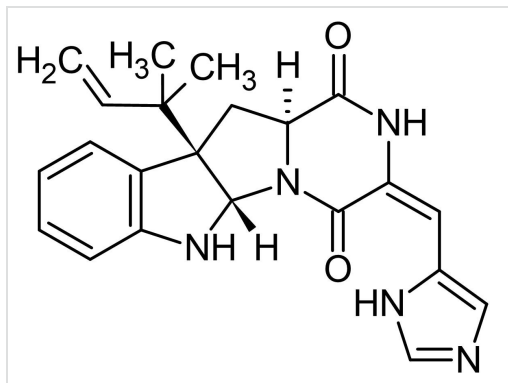
Chemical Structure - Roquefortine C, Neurotoxin (ab144345)
