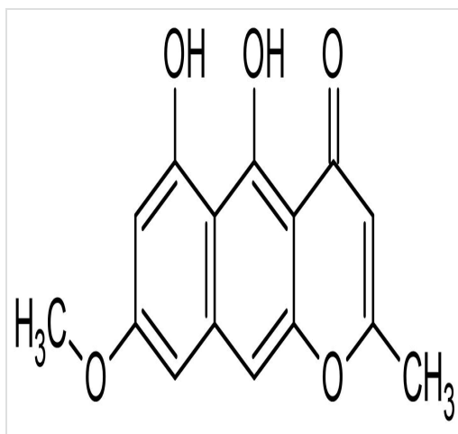
Chemical Structure - Rubrofusarin, tyrosinase inhibitor (ab144348)
