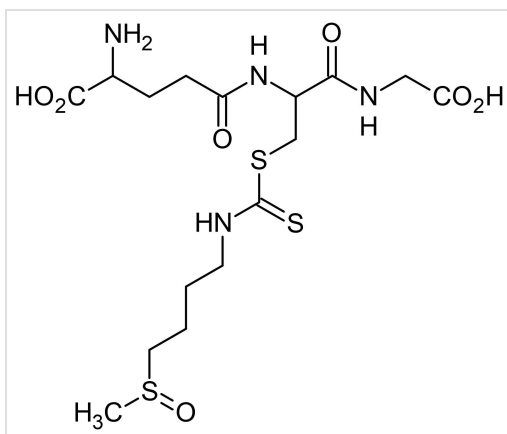
Chemical Structure - S-(N-Methylsulfinylbutylthiocarbamoyl)-glutathione, Sulforaphane glutathione conjugate (ab142756)
