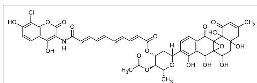
Chemical Structure - Simocyclinone D8, Topoisomerase I and II inhibitor (ab144362)
