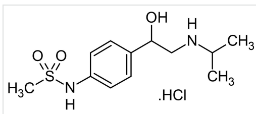
2D chemical structure image of ab142370, Sotalol hydrochloride, beta adrenoceptor antagonist
