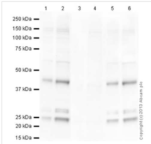
Western blot - Anti-SOX2 (GlcNAc S248) antibody (ab136167)
