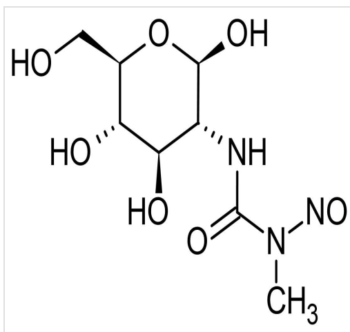
Chemical Structure - Streptozocin, Pancreatic beta- cell toxin (ab142155)
