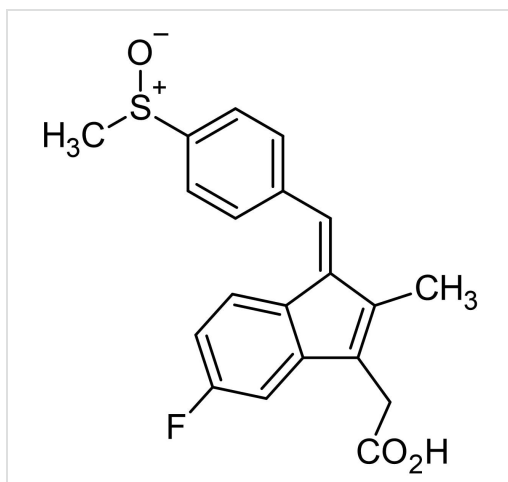
Chemical Structure - Sulindac, non-steroidal anti-inflammatory agent (ab142950)
