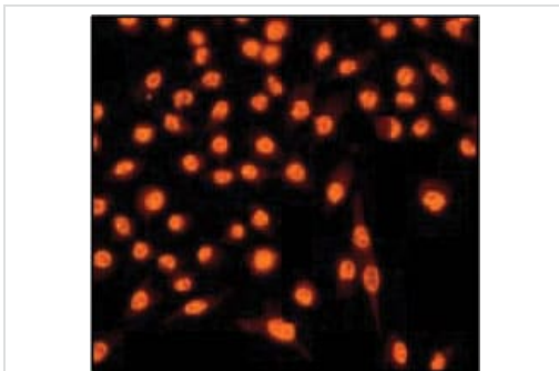
Immunocytochemistry/ Immunofluorescence - Anti-Sumo 1 antibody [Y299] - ChIP Grade (ab32058)
