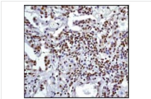
Immunohistochemistry (Formalin/PFA-fixed paraffin-embedded sections) - Anti-Sumo 1 antibody [Y299] - ChIP Grade (ab32058)
