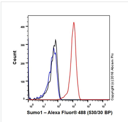
Flow Cytometry - Anti-Sumo 1 antibody [Y299] - ChIP Grade (ab32058)
