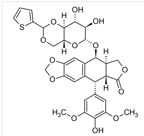
Chemical Structure - Teniposide, Topoisomerase II inhibitor (ab142643)
