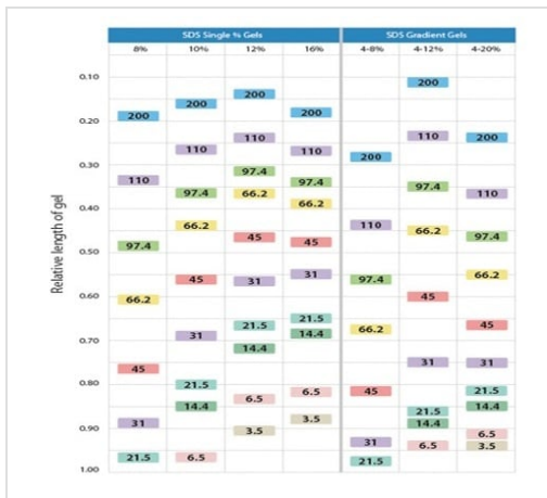
SDS-PAGE - TEO-Tricine Precast Gels - RunBlue™ (4-20%, 2-well, 10x10cm) (ab270461)
