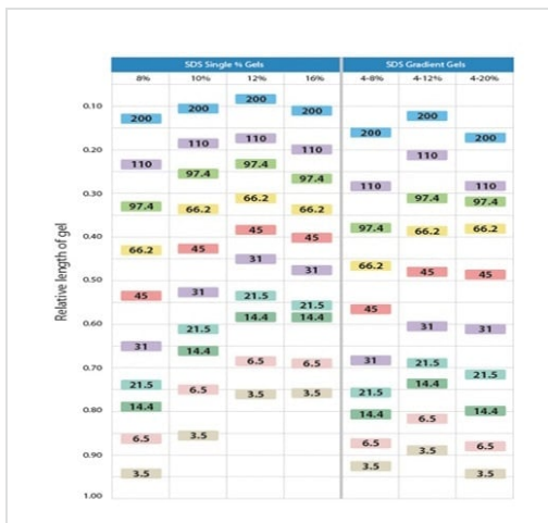
SDS-PAGE - TEO-Tricine Precast Gels - RunBlue™ (4-20%, 2-well, 10x10cm) (ab270461)
