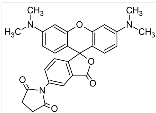
Chemical Structure - Tetramethylrhodamine-5-maleimide, Labeling reagent for protein thiols (ab145443)
