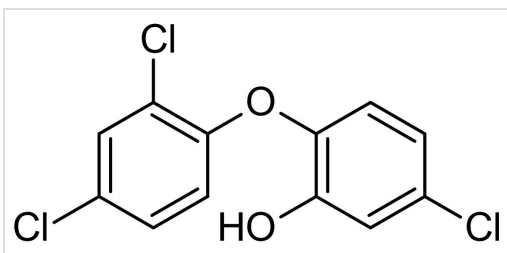
Chemical Structure - Triclosan, Anti-inflammatory activities (ab145584)
