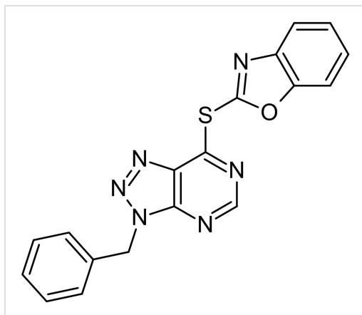
Chemical Structure - VAS 2870, NADPH oxidase inhibitor (ab145209)
